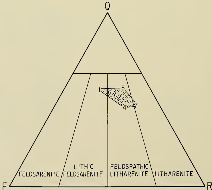
Fig. 5. QFR diagram for sandstones from Cupala Creek Formation. Specimens numbered in stratigraphic order on type section (Fig. 3).
